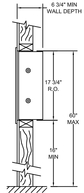
FINISHED FLOOR (RECESS MOUNT)
